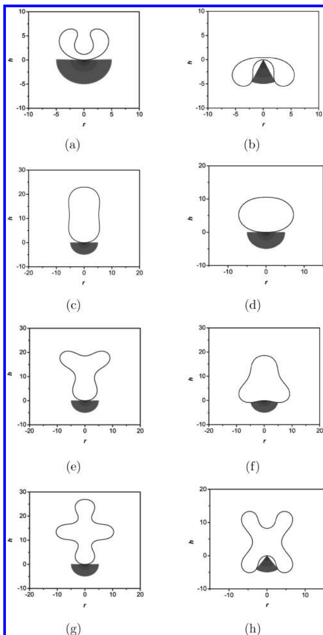
Figure 2. Typical stationary solutions of vesicle anchored by rigid rod outside, including shapes of the vesicle and segment distributions of the anchored rod. The shape of the vesicle is represented by the solid curve, and the density of the polymer chain is drawn in gray scale on a logarithmic scale. The radial (horizontal) and height axes are scaled by Nb . In all cases, we use N_p = 100 , c_0 = 0 , \chi = 0 , \eta = 0 . (a) \kappa = 15 , \Delta p = 0.0036 , \lambda = -0.027 . (b) \kappa = 10 , \Delta p = 0.0024 , \lambda = -0.02 . (c) \kappa = 3 , \Delta p = 0.00072 , \lambda = -0.0132 . (d) \kappa = 5 , \Delta p = 0.0012 , \lambda = -0.02 . (e) \kappa = 2 , \Delta p = 0.00048 , \lambda = -0.008 . (f) \kappa = 2 , \Delta p = 0.00048 , \lambda = -0.0096 . (g) \kappa = 1.5 , \Delta p = 0.00036 , \lambda = -0.006 . (h) \kappa = 5 , \Delta p = 0.0012 , \lambda = -0.0156 .
