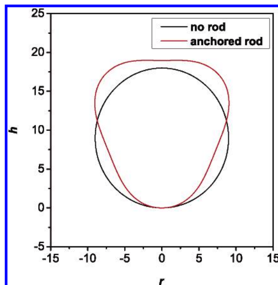
Figure 3. Transformation of vesicle shape after anchored rod. In all cases, we use c_0 = 0 , \chi = 0 , \eta = 0 , \kappa = 5 , \Delta p = 0.0012 , \lambda = -0.02698 . The rod length is N_p = 100 .
