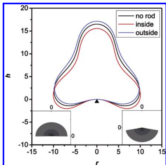
Figure 5. Shape of vesicle anchored by rigid rod outside ( \zeta > 0 ) and inside ( \zeta < 0 ). N_p = 100 , \kappa = 10.0 , c_0 = 0 , \Delta p = 0.0024 , \chi = 0 , \eta = 0 , and \lambda \sim -0.045 is set to keep the area of vesicle to be constant.
